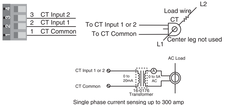
Figure 10b — Single Phase
