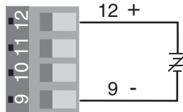
Figure 8d — Input 2, 0 to 10V DC (dc) Process Input
