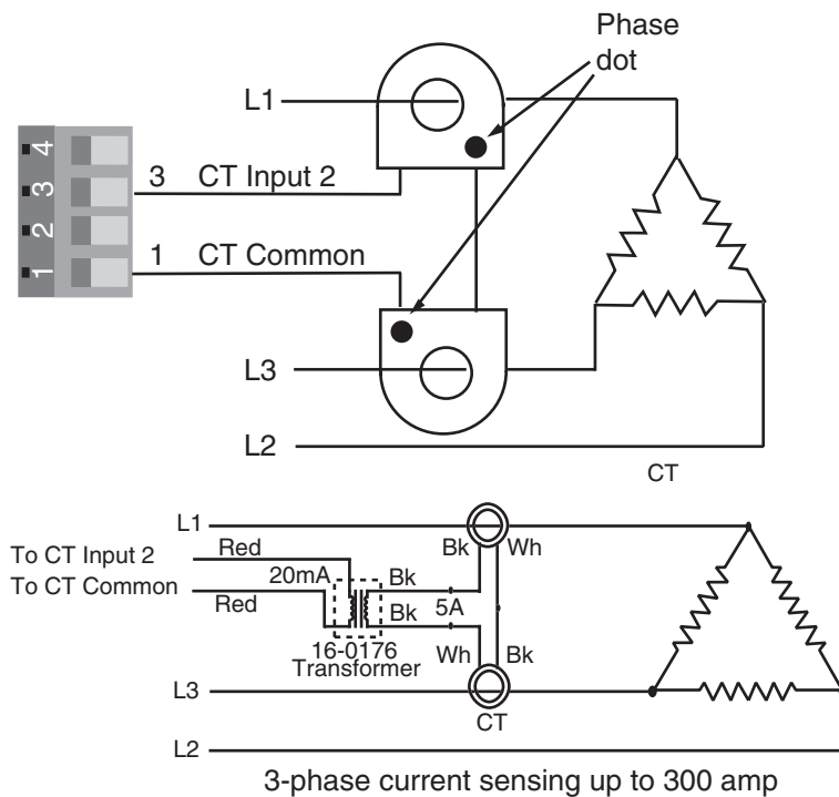
Figure 12b — Current Transformer Input 2, Three Phase
