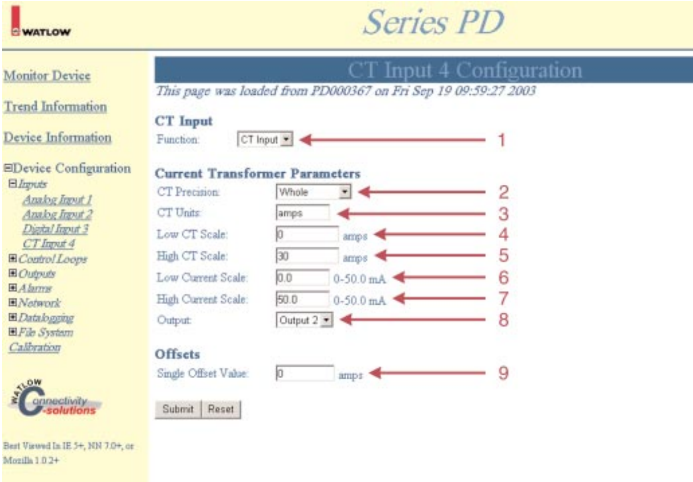
Figure 33 — CT(current transformer) Input Configuration Web Page Example
