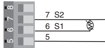
Figure 8b — 3-Wire RTD Input 2 (100 \Omega DIN curve 0.00385 \Omega/\Omega/^\circ\text{C} )
