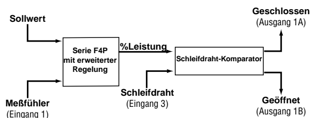
Abbildung 7.17a — Schleifdraht-Feedback.
