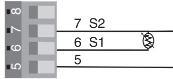
Figure 8b — 3-Wire RTD Input 2 (100 Ω DIN curve 0.00385 Ω/Ω/°C)
