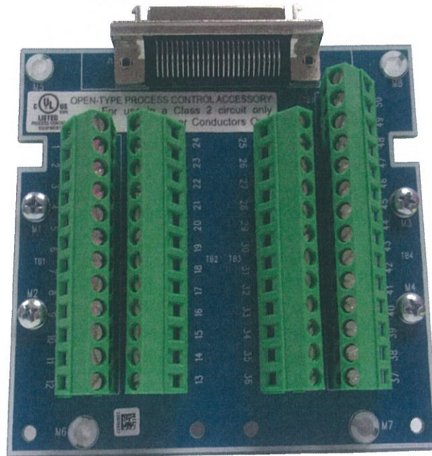
TB50 Breakout Connector Board
